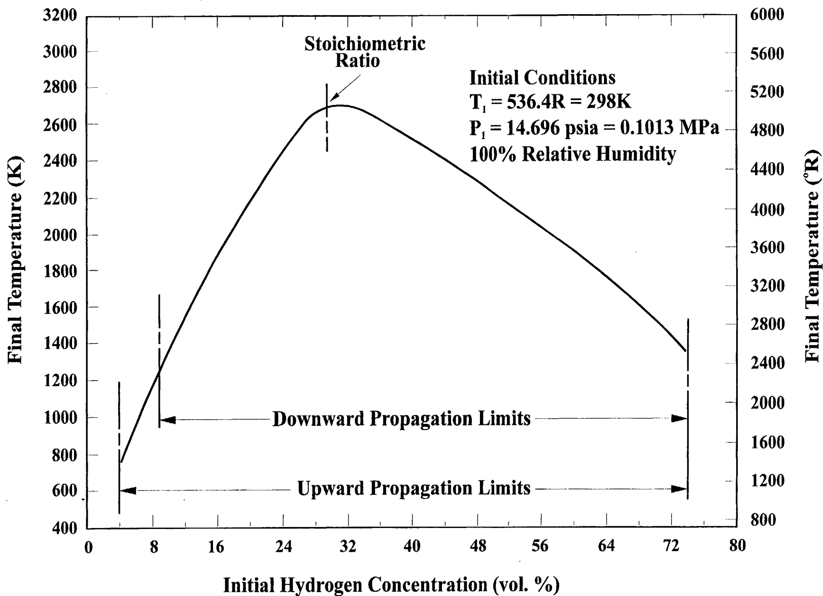
Figure 4A-2 Theoretical adiabatic, constant-volume combustion temperature for hydrogen: air mixtures
