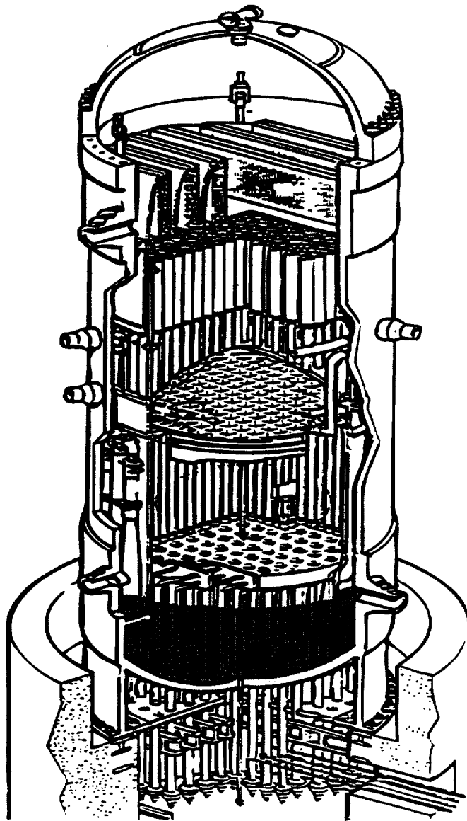
Figure 3.7-7 Regional above core plate would be dry during structural degradation
