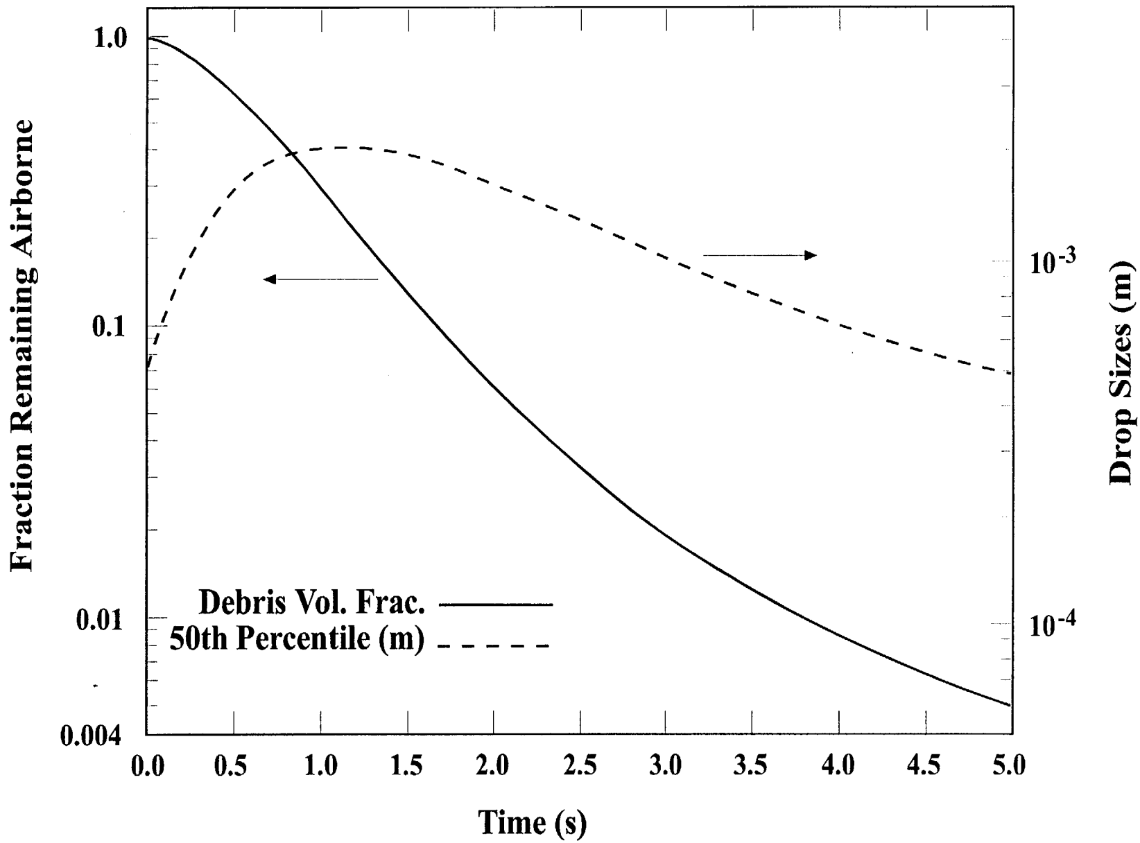
Figure 4.5-4 Estimated median particle size versus time
