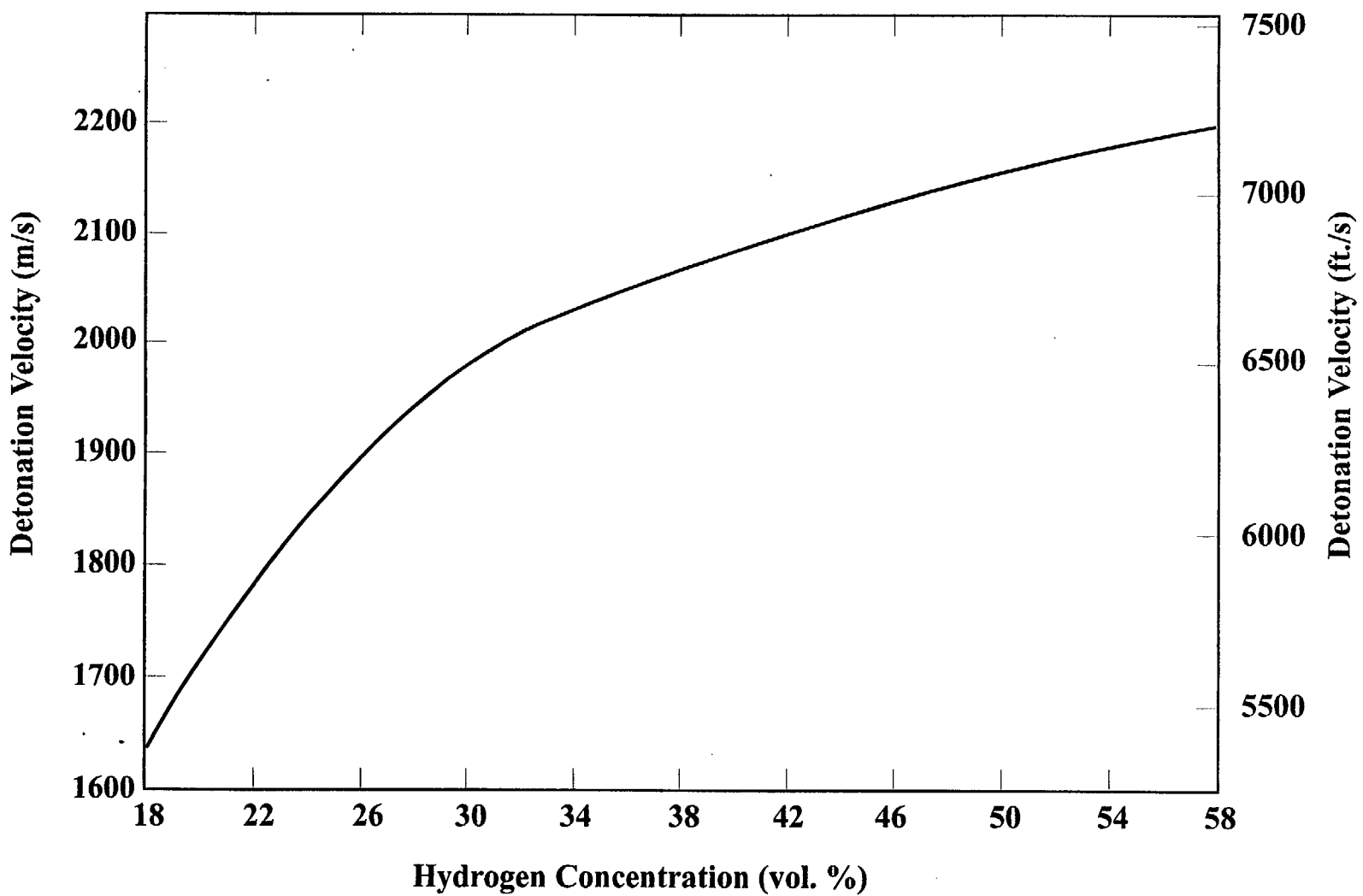
Figure 4.6-9 Theoretical detonation velocities for hydrogen : air mixture
