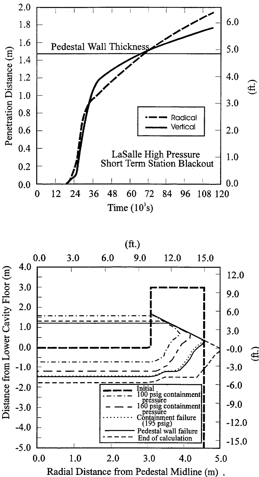
Figure 4.4-2 Calculations of concrete attack in a BWR Mark II containment during a station blackout sequence
